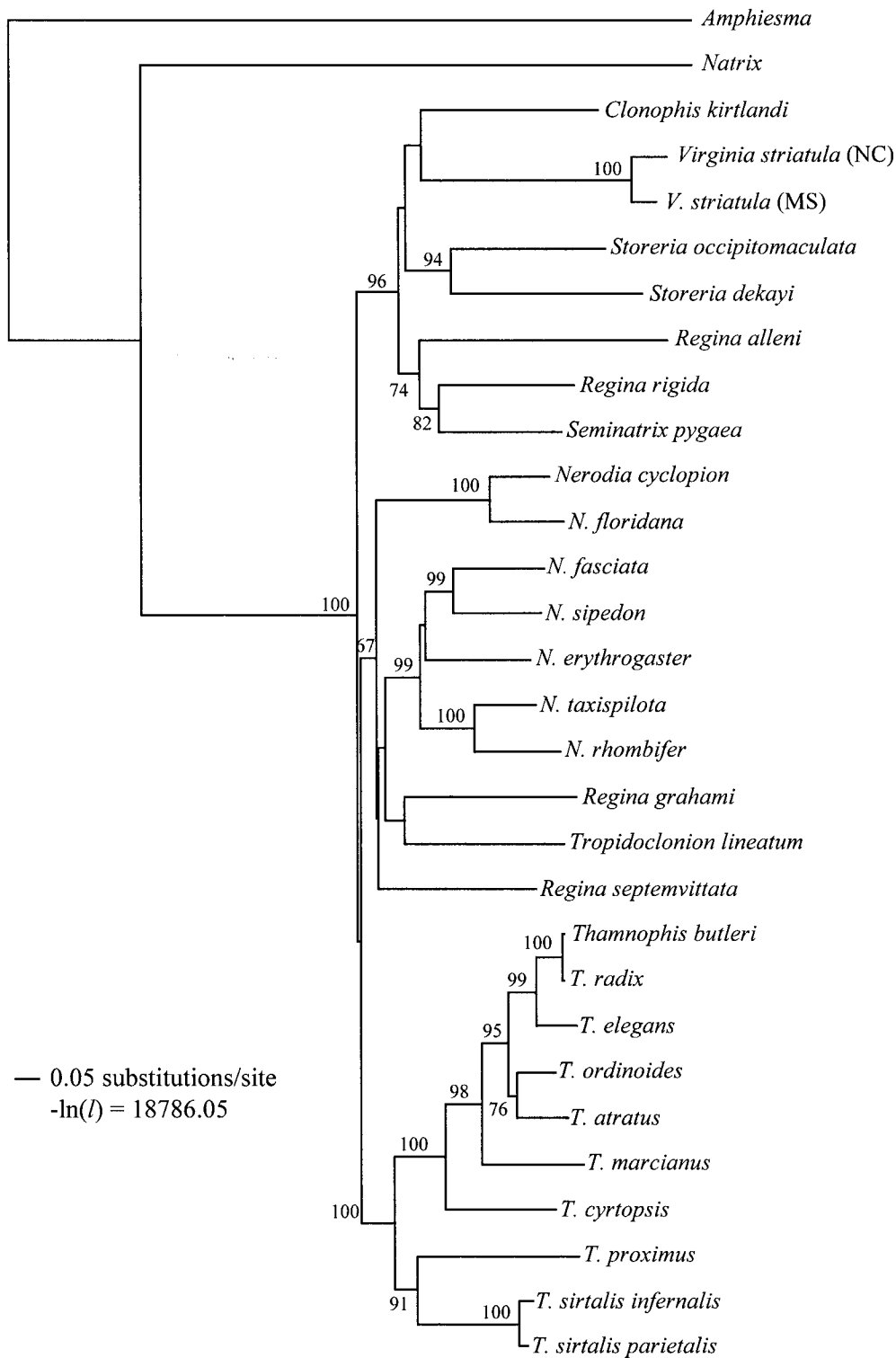
FIG. 3. Maximum-likelihood tree. Shown is the single most likely tree ( -\ln(l) = 18786.05 ) recovered under a GTR model with invariant sites and rate heterogeneity among sites. Numbers at nodes represent percentage of bootstrap replicates supporting that node. Topologies of trees recovered under maximum-parsimony and maximum-likelihood are largely similar, although relationships within the semifossorial clade differ between the two types of analyses.
