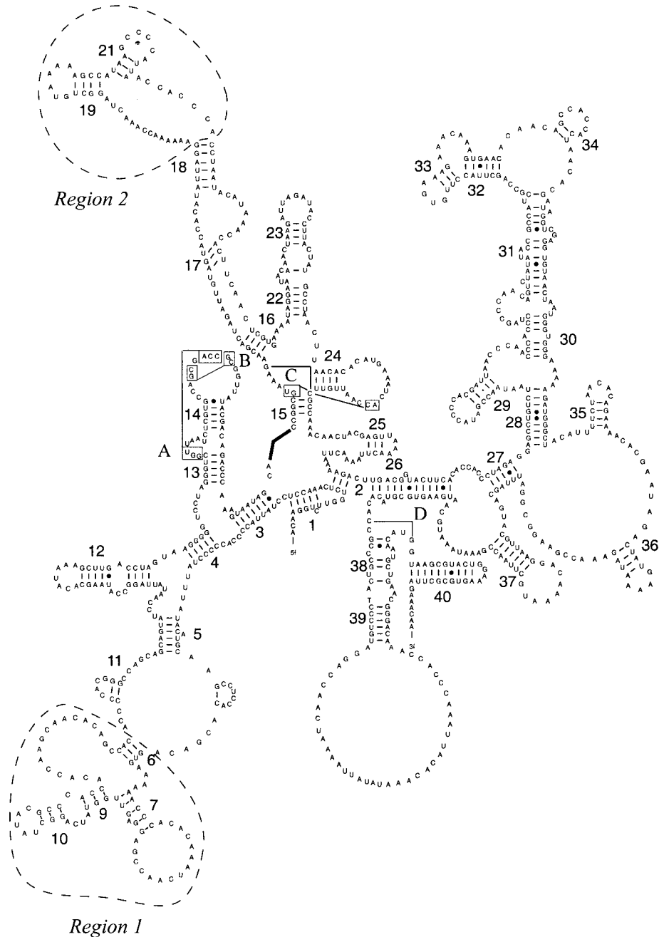
FIG. 1. Snake 12S ribosomal RNA model. Shown is the secondary structure model for thamnophiine 12S RNA illustrated with Thamnophis marcianus . Stem numbering follows Springer and Douzery (1996). Dashes indicate base pairing; dots indicate U-G (non-canonical) base pairs. Uppercase letters refer to predicted tertiary interactions (from Gutell, 1994). Dotted lines indicate two regions that could not be aligned unambiguously to either mammal (Springer and Douzery, 1996) or bird (Mindell et al. , 1997) models.
