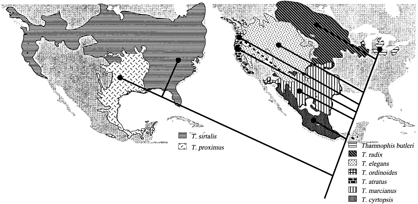
FIG. 7. Biogeography of Thamnophis . Ranges shown are approximate and taken from Rossman et al. (1996). The basal members of one main lineage of garter snakes have a Mexican and southern U.S. distribution, whereas the more distal species in the tree are found northward and westward. This supports the hypothesis that at least one major lineage of garter snakes originated in Mexico. The biogeographic pattern of the lineage containing T. sirtalis is consistent with the hypothesis of a second invasion of North America, although taxon sampling is too sparse to generate high confidence for this scenario.
