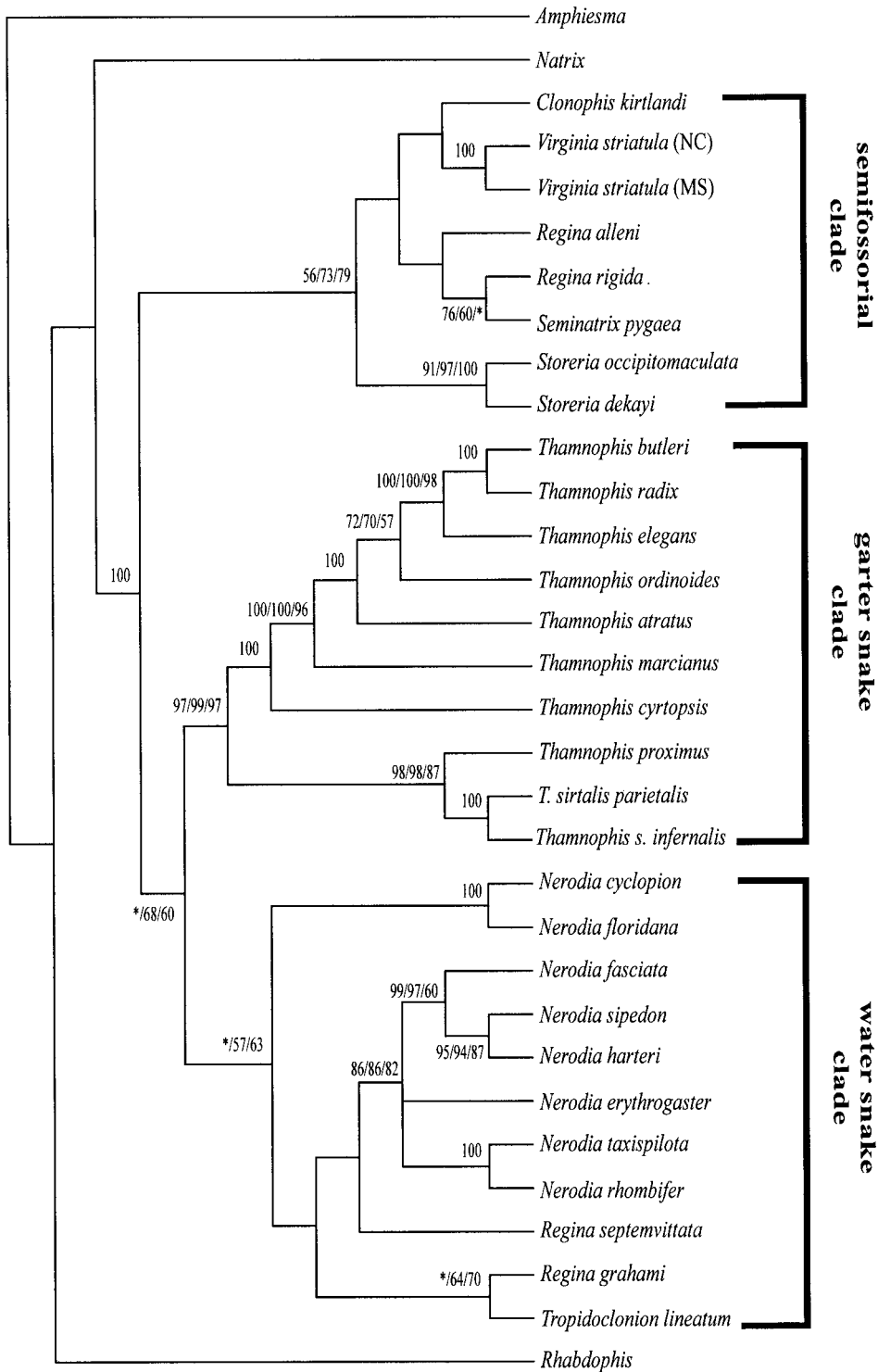
FIG. 2. Consensus of two equally most parsimonious trees. Tree length = 3665 steps; Consistency Index = 0.428; Retention Index = 0.458. Numbers at nodes represent percentage of bootstrap replicates supporting that node under three different weighting schemes: equal weights, third position transitions downweighted by one half relative to other changes, and third position transitions excluded. Three main clades are recovered, although bootstrap support is generally weak for the water snake clade. The genus Regina is polyphyletic and Nerodia is paraphyletic with respect to other thamnophiines.
