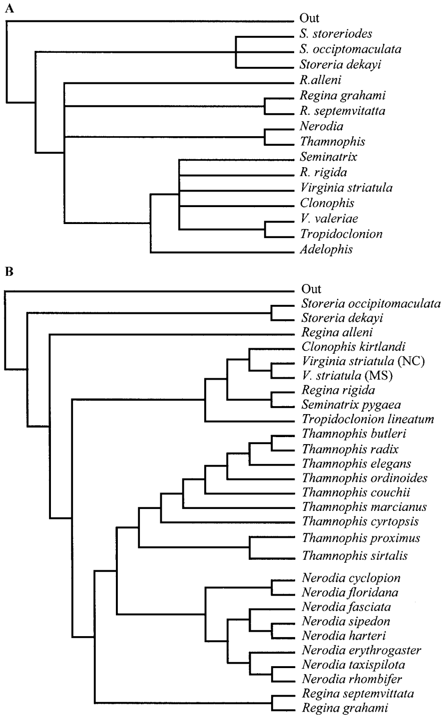
FIG. 6. Allozyme tree and allozyme constraint tree. (A) Phylogeny of the Thamnophiini based on allozyme data (Lawson, 1985). (B) Most parsimonious tree recovered under the topological constraint of the allozyme tree. Tree length = 4460 steps; Consistency Index = 0.352. The constrained tree is 42 steps longer than the unconstrained most parsimonious tree.
