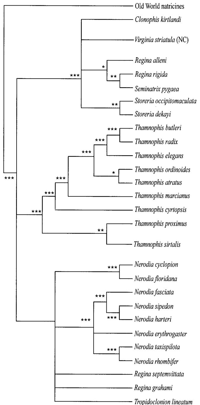
FIG. 5. Preferred phylogenetic hypothesis for thamnophiines. Tree shown is based on the maximum-likelihood tree (Fig. 6) with poorly supported nodes (bootstrap proportions <65%) collapsed. Our data resolve relationships at many levels of the tree and suggest that the thamnophiine radiation is composed of three main lineages. Relationships among these lineages are uncertain as are relationships at the base of the water snake and semifossorial clade. ***ML bootstrap support \geq 95 ; **ML bootstrap support \geq 80 ; *ML bootstrap support \geq 70 .
