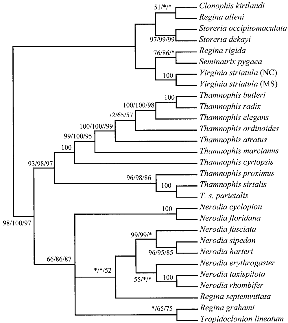
FIG. 4. Strict consensus of two equally most parsimonious unrooted networks of ingroup taxa. Tree length = 2795; Consistency Index = 0.438. Numbers at nodes represent percentage of bootstrap replicates supporting that node under three different weighting schemes: equal weights, third position transitions and loop transversions downweighted by one half, and third position transitions and loop transversions downweighted to 0. Asterisks indicate that bootstrap support for that node was less than 70 under that weighting scheme. Without outgroups, bootstrap support dramatically increases for the bipartition between the semifossorial group and the rest of the thamnophiines and increases for the bipartition between the water snakes clade and the rest of the thamnophiines. This result suggests that long branch attraction may be contributing to root instability in the rooted analysis.
