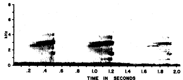
FIGURE. Audiospectrogram of call of Pseudacris brachyphona : Little Walker Creek, Pulaski County, Virginia, 29 March 1975; no temperature or voucher specimen.
